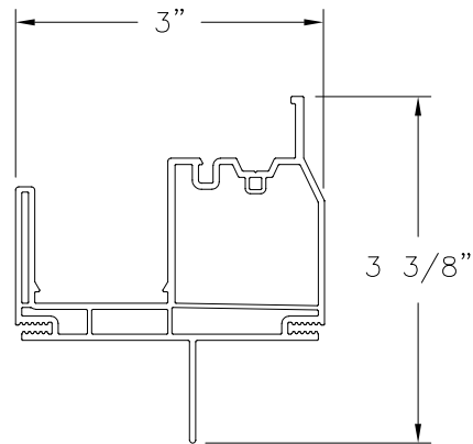
MAIN FRAME (9204) EXTRUDED RIGID PVC
