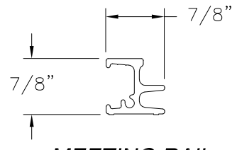
MEETING RAIL REINFORCEMENT (10635) ALUMINUM 6005-T5
